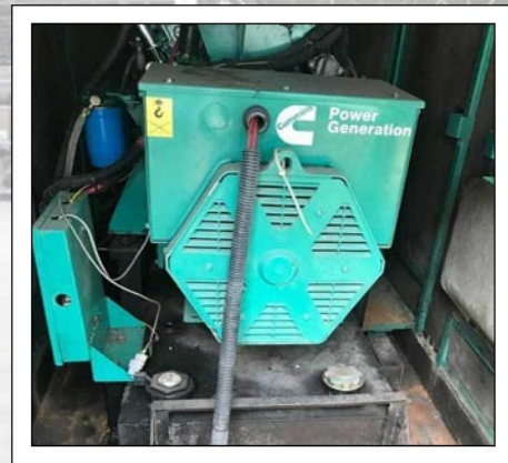
380 kVA Used Cummins Diesel Generator Set and 25 kVA Used Tata Cummins Diesel Generator Set
